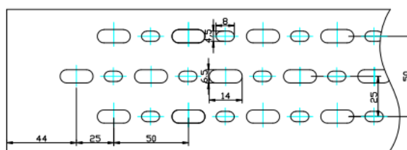
Suitable for wire slot width 75mm and above
